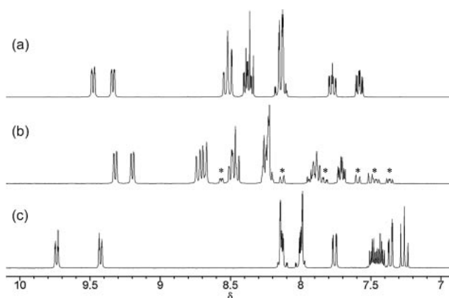
Figure 7. 1 H NMR (300 MHz) spectra of (a) 4 in methanol- d 4 , (b) 4 in DMSO- d 6 , and (c) 5 in DMSO- d 6 . Asterisks denote the signals of the free ligand L 1 .
