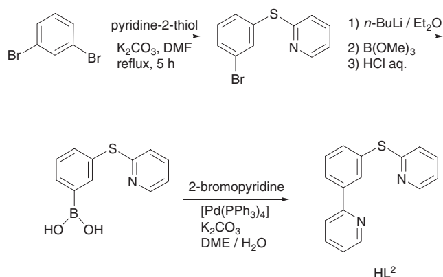
Scheme 2. Synthesis of a precursor for the N,C,N -tridentate ligand L 2 .
