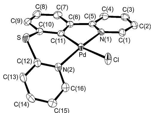
Figure 5. ORTEP drawing of 5 with thermal ellipsoids at the 50% probability level. Hydrogen atoms are omitted for clarity.
