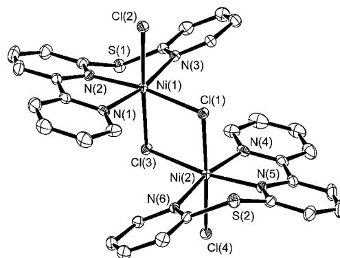
Figure 2. ORTEP drawing of 2 with thermal ellipsoids at the 50% probability level. Hydrogen atoms are omitted for clarity.
