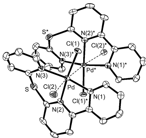
Figure 4. ORTEP drawing of 4 with thermal ellipsoids at the 50% probability level. Hydrogen atoms are omitted for clarity.
