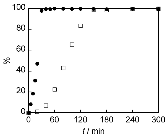
Figure 8. Time course of the yields of methyl trans -cinnamate for the Mizoroki–Heck reactions of iodobenzene (2 mmol) and methyl acrylate (3 mmol) catalyzed by 4 (0.1 mol %, ●) and 5 (0.1 mol %, □). The reactions were performed in N,N -dimethylformamide (10 mL) at 110 °C, using triethylamine (3 mmol) as a base.
