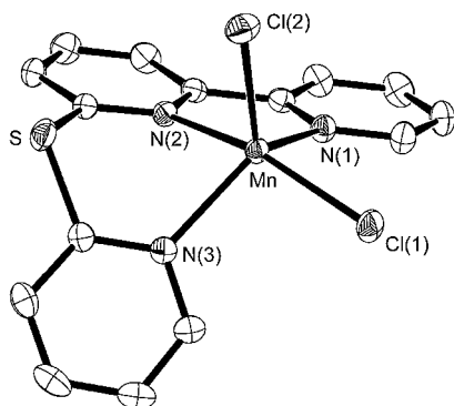
Figure 1. ORTEP drawing of 1 with thermal ellipsoids at the 50% probability level. Hydrogen atoms are omitted for clarity.
