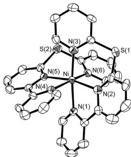
Figure 3. ORTEP drawing of 3 with thermal ellipsoids at the 50% probability level. Hexafluoroantimonate anions and hydrogen atoms are omitted for clarity.
