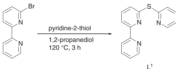
Scheme 1. Synthesis of the N,N,N -tridentate ligand L 1 .
