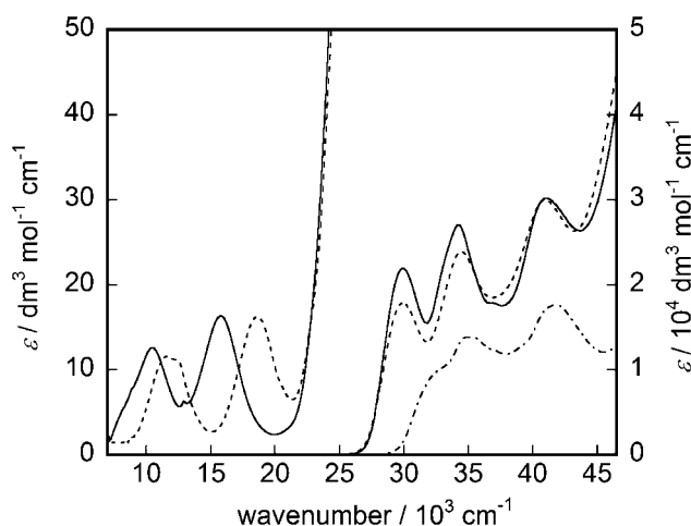
Figure 6. Absorption spectra of 2 in methanol (—), 3 in acetonitrile (---), and \text{L}^1 in methanol (-.-).
