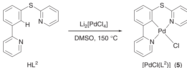
Scheme 3. Synthesis of the palladium complex [\text{PdCl}(\text{L}^2)] ( 5 ).
